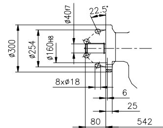
Mounting flange for multi-turn actuator G4- DIN 3210
