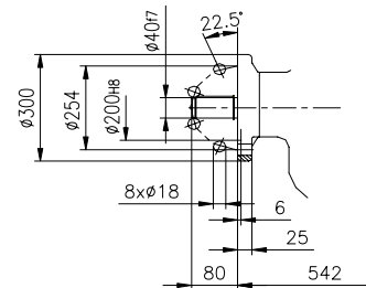
Mounting flange for multi-turn actuator F25- ISO 5210
