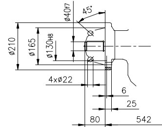
Mounting flange for multi-turn actuator F16- ISO 5210 G3-DIN 3210
